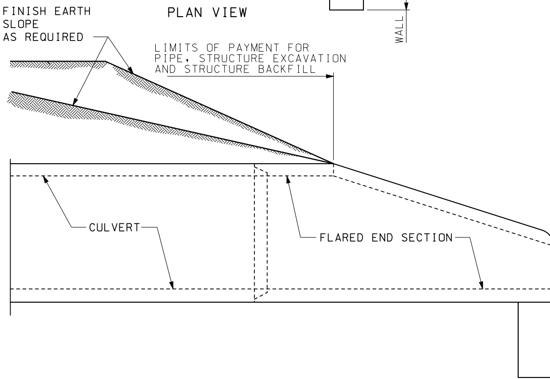
INSTALLATION DETAILS
